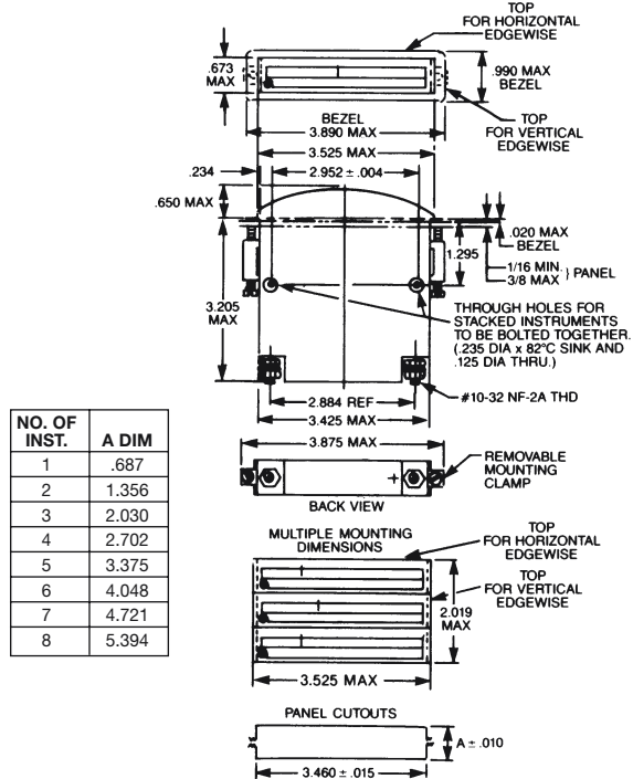
Fig. 19. Outline Dimensions for 3½-inch Type 288 meters
