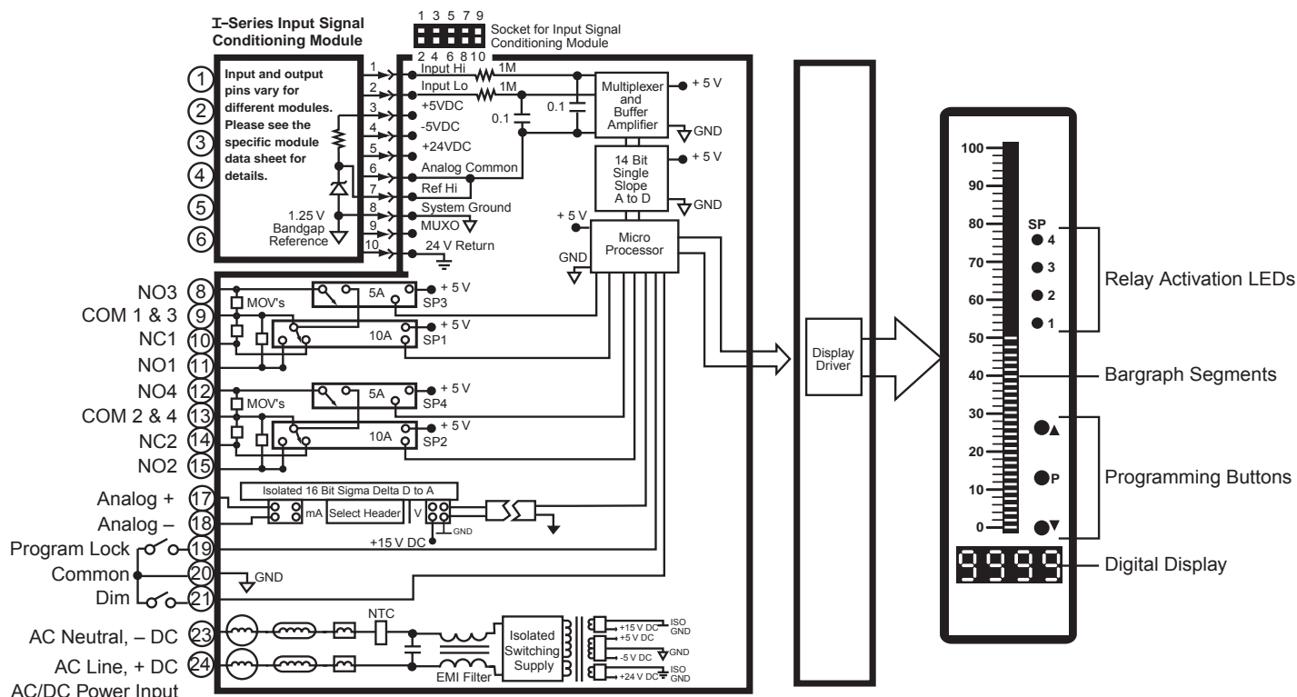
FL-B101D40 Functional Diagram
