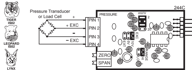
ISO6: Pressure/Load Cell Ext Exc., 20/2mV/V, 4-wire
