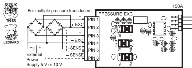
ISO5: Pressure/Load Cell 20/2mV/V, 5/10V Exc 4-wire
