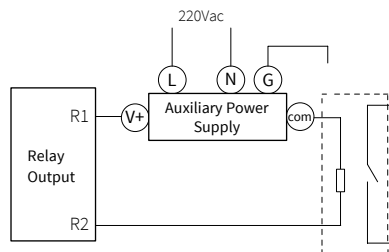
Relay output
