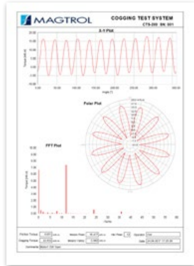
Above is an example of a compiled report that can be used as a certificate. In addition to the measured data, the report can contain X-Y, polar and FFT graphs.
