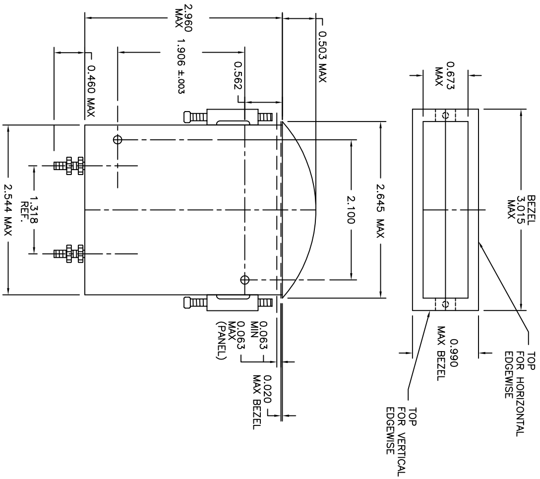
FIG. 18. OUTLINE DIMENSIONS FOR 2 1/2 INCH TYPE 287 METERS REV 1/22/03 (DWG 3151K77)
