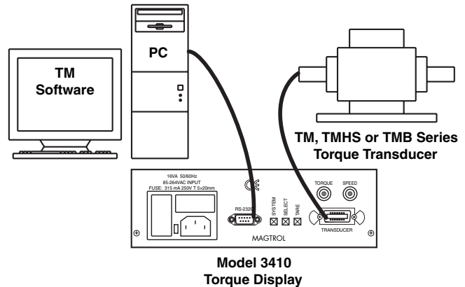
PC-Based System Configuration Torque Transducer with Model 3410 Display and Torque Software
